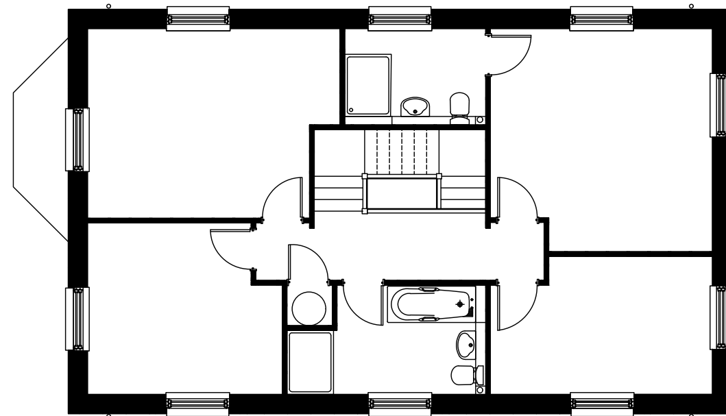
SECOND FLOOR PLAN 1:100
