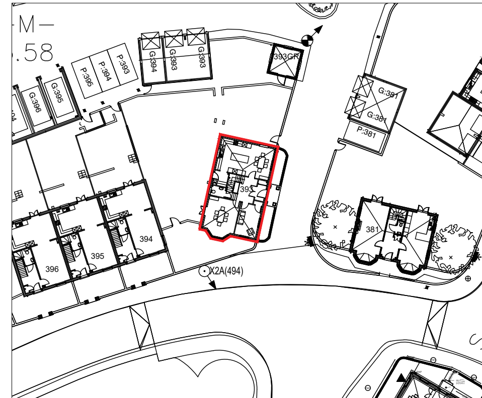
Location Plan 1:500
