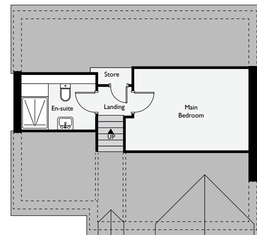
Second Floor Layout
