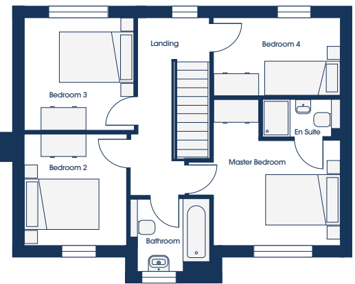
STANDARD FLOORPLAN
