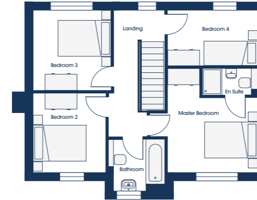
STANDARD FLOORPLAN
